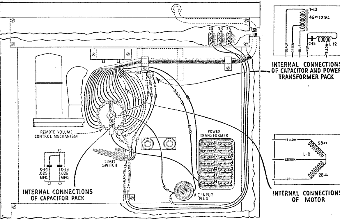
Wiring Diagram of Remote Volume Control Panel
